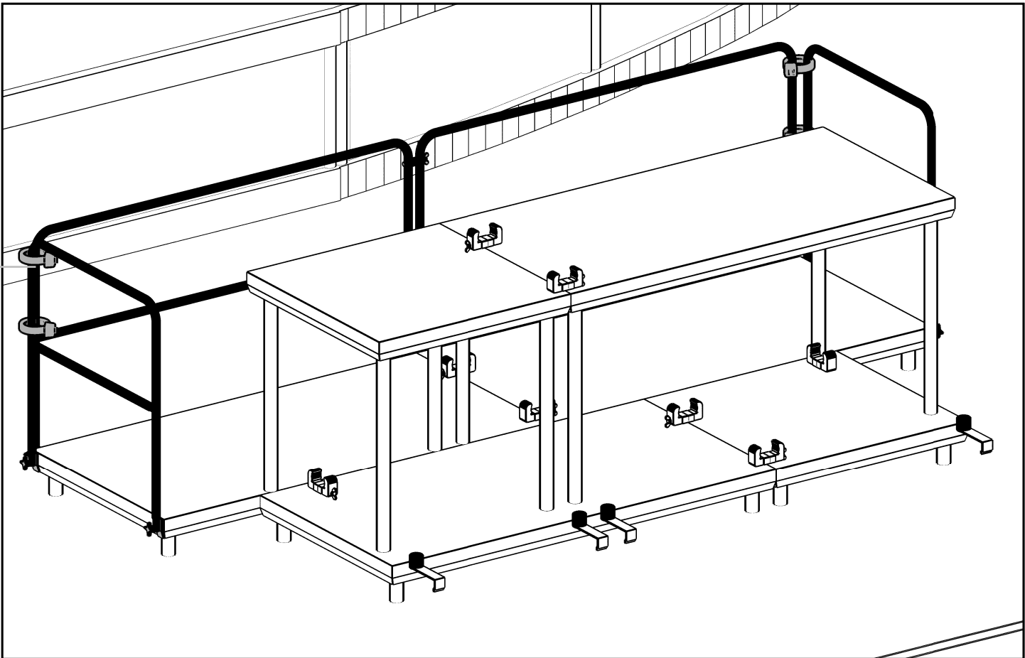
DJ Setup 9 - 3m Booth in Hall Center 3m DJ-Booth with 4m Riser
